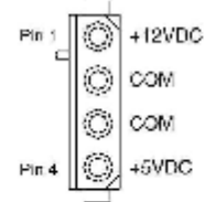
Peripheral Power Connector
